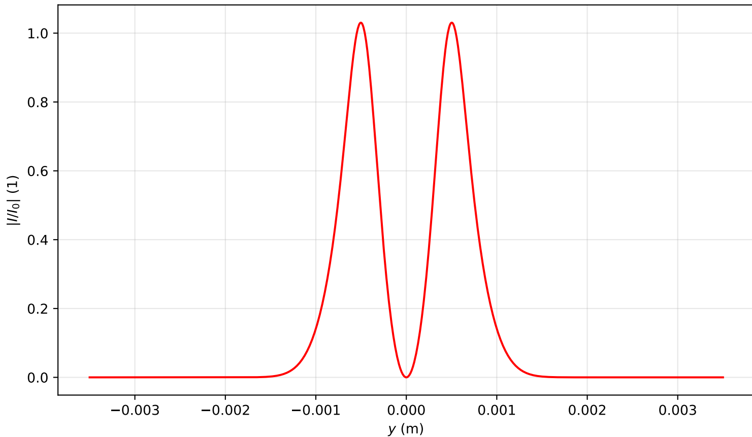
Intensity profile I(x=0, y, z=0.318)/I_0 , P_{in}=5.0P_{cr} , artificial time
